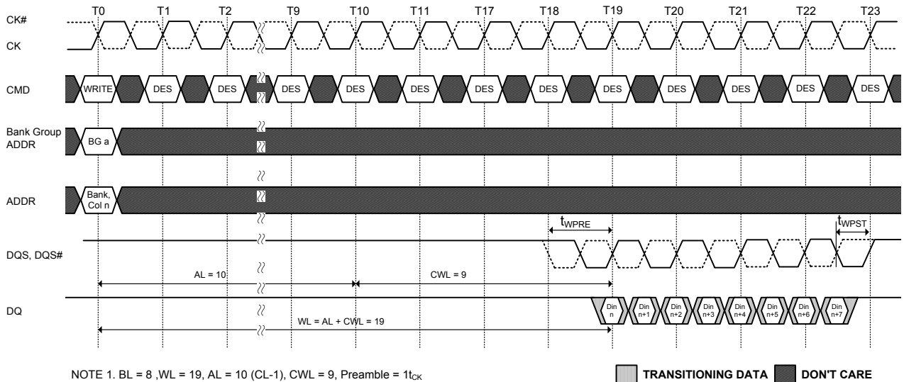
Figure 133. WRITE Burst Operation WL = 9 (AL = 0, CWL = 9, BL8)
