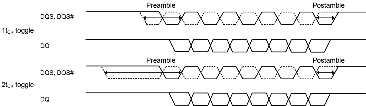
Figure 87. WRITE Postamble
