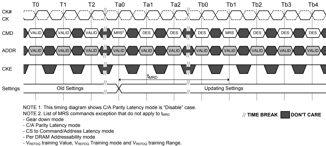
Figure 6. t_{MRD} timing
