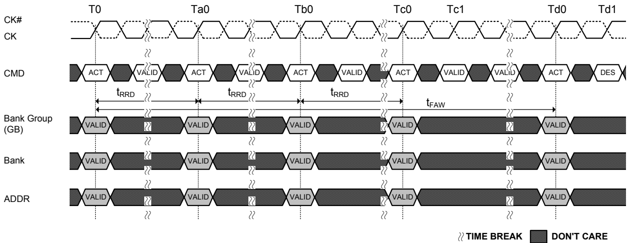
Figure 77. t_FAW Timing
