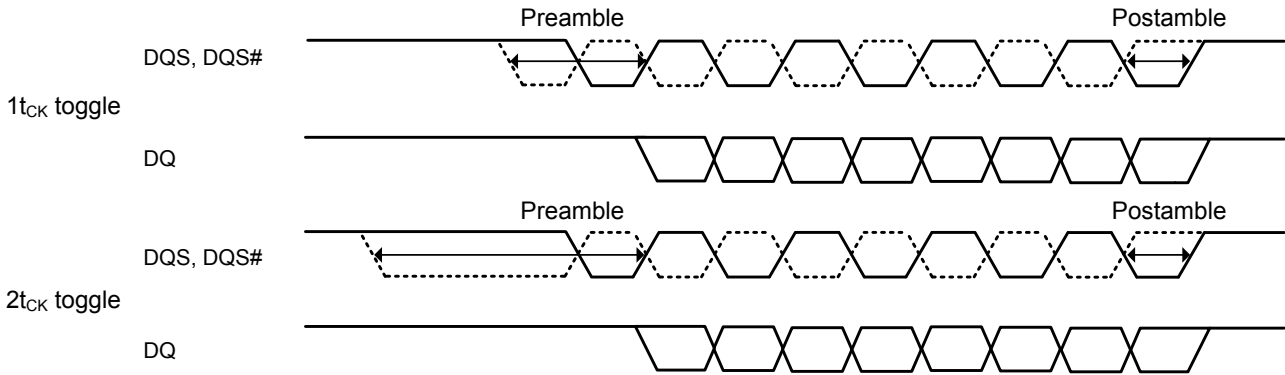
Figure 86. READ Postamble
